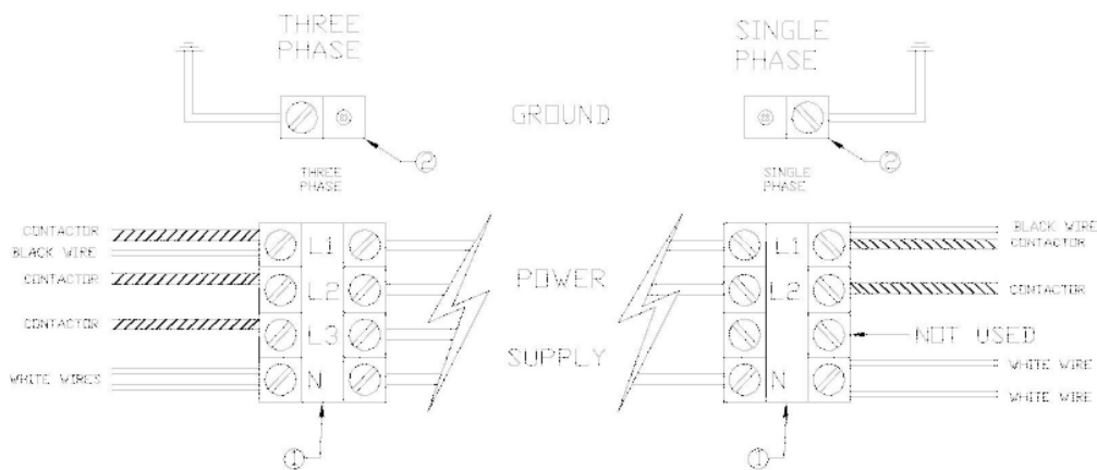
Fig. #2 – Power Supply Connections
