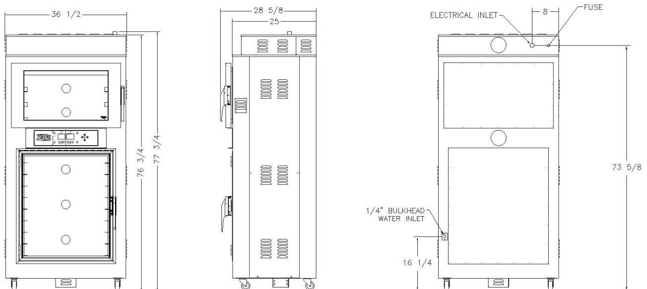
Fig. #1 - Installation
