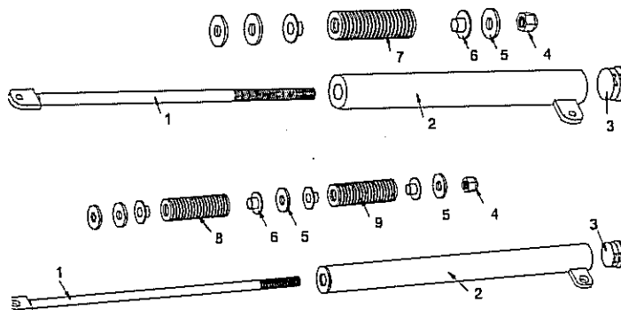
Fig. 6.1: Actuator Assembly Diagram
