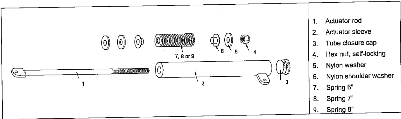
Fig. 3.1: Actuator Components & Assembly
