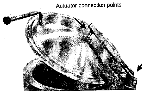
Fig. 3.2: Removing/Installing Actuators
