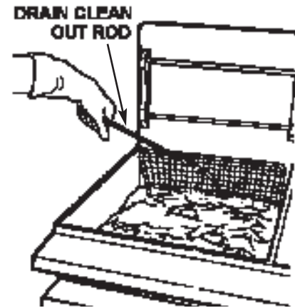
FIGURE 3. REMOVE SCREEN OVER TUBES/ELEMENTS
