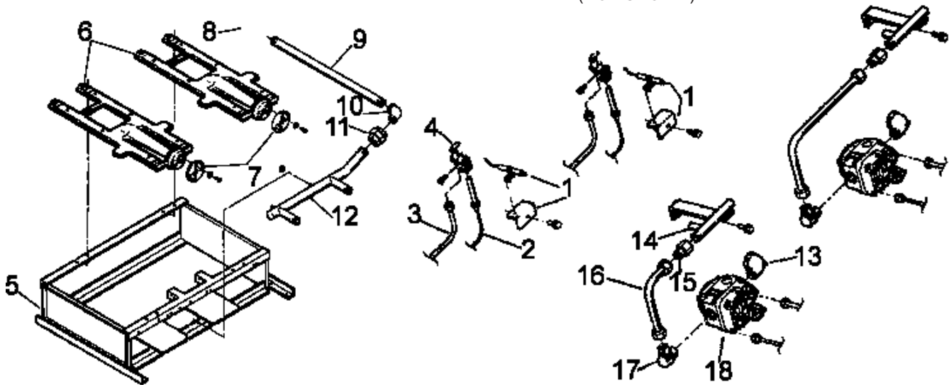
Figure 6-3 Natural and Propane Gas Heating Systems
