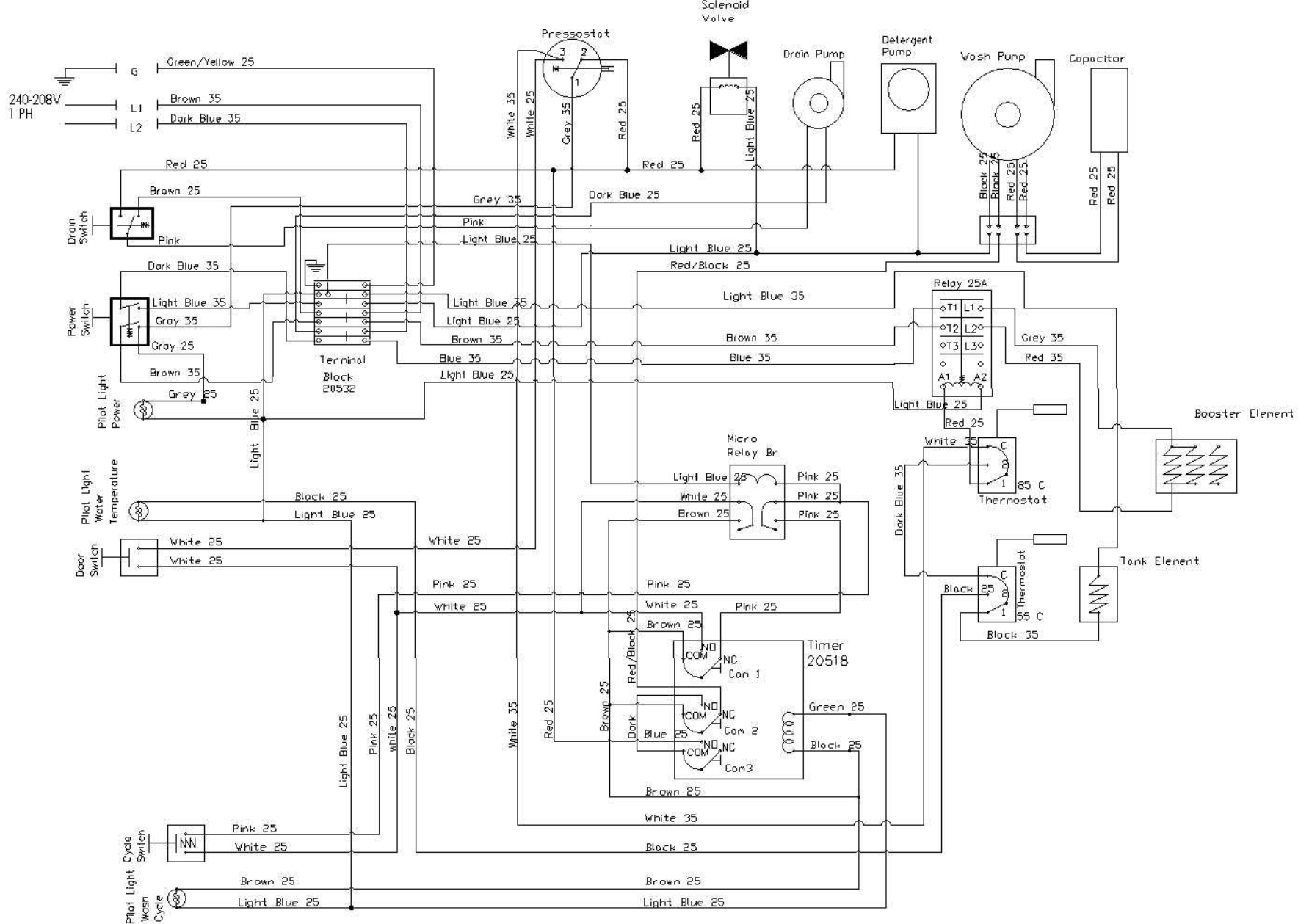
Electrical diagram on Jet Tech F 18 DP Actual may be diferent The number after each wire color represent the wire thickness with insulation 25 = 2.5mm 35 = 3.5mm
