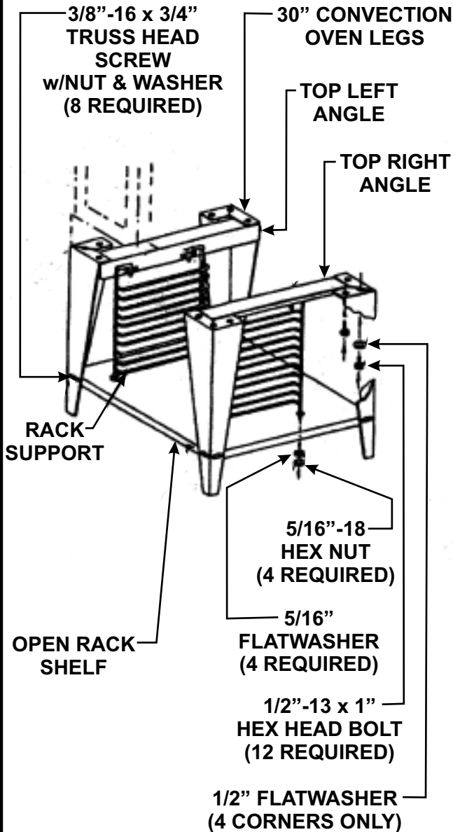
Fig. 4 ASSEMBLY OF LEGS (SHOWN WITH OPEN RACK STAND)
